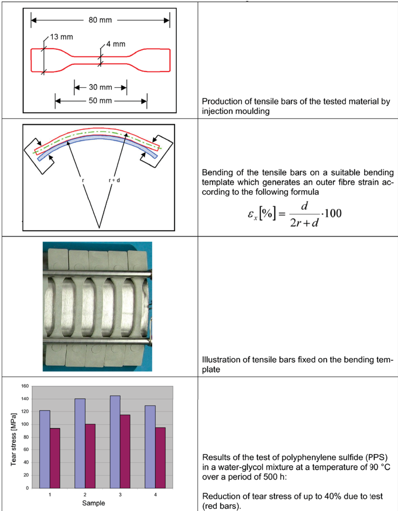
Figure 62: Realisation of a test for environmental stress cracking
