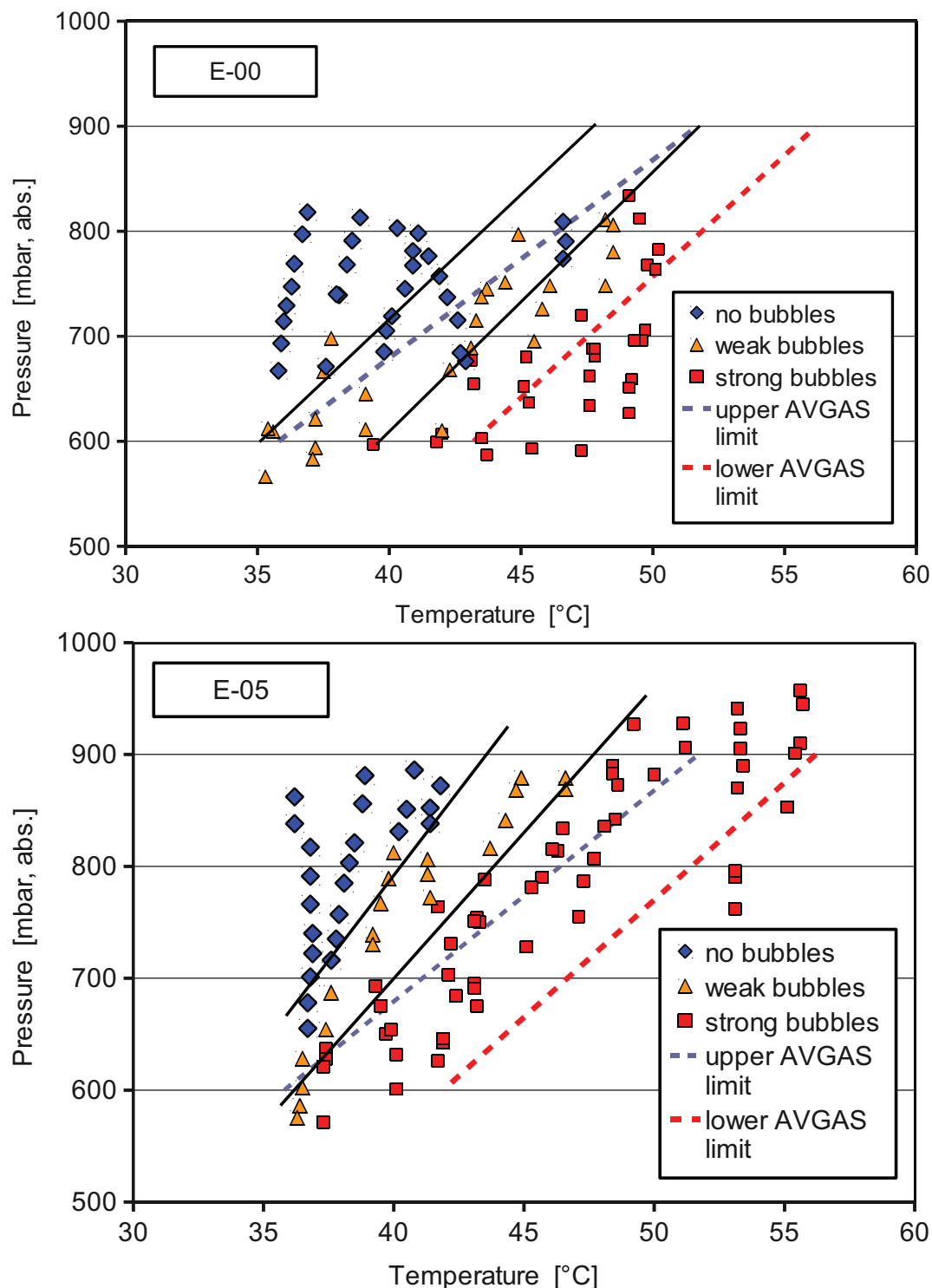
Figure 49: Bubble sensor readouts for a \{p,T\} scan of E-0 (top) and E-5 (bottom). Blue diamonds indicate a readout S < 0.3 V, orange triangles a value 0.3 \text{ V} < S < 0.7 V, red squares indicate S > 0.7 V. Averaged region borders are sketched as black lines. Respective borders for AVGAS (cf. Fig. 48) are additionally shown as dashed lines.
